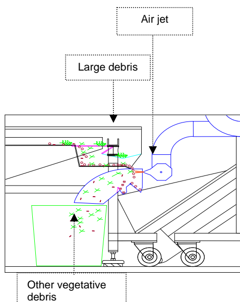
Air jet functions at end of distribution table.
